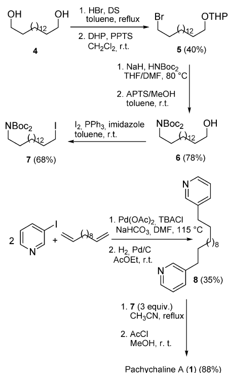
Scheme 1. Total synthesis of pachychaline A ( 1 ).
