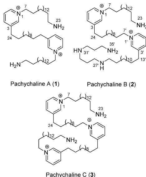
Figure 1. Structures of pachychalines A (1), B (2), and C (3).
